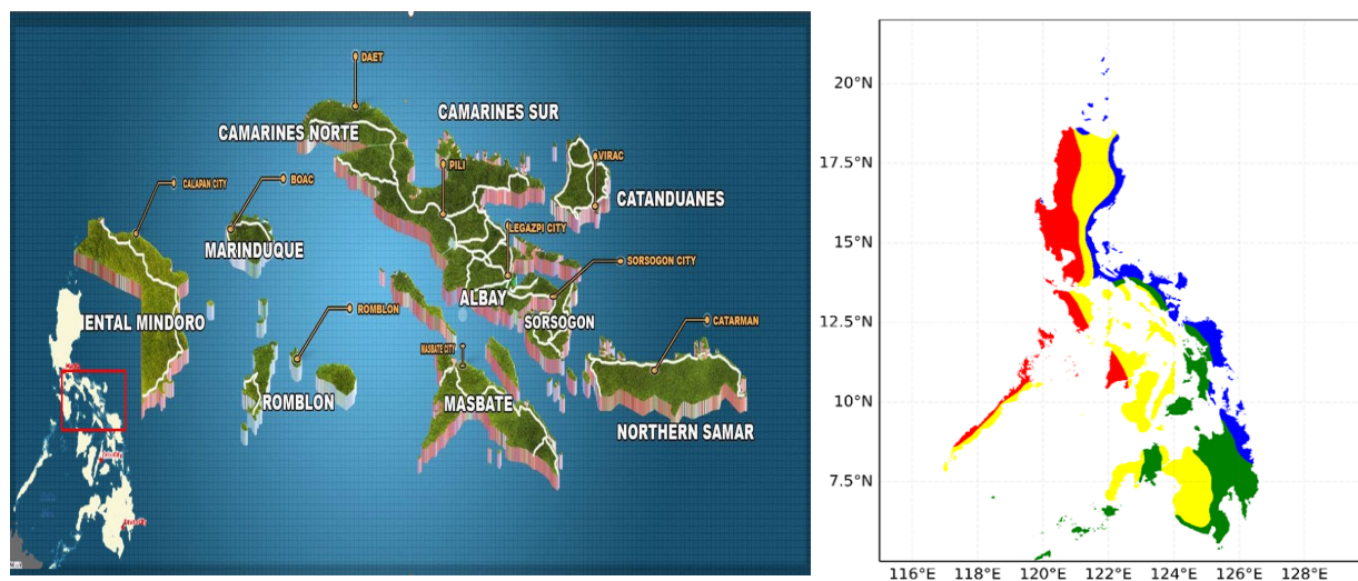
Figure 1 Southern Luzon PRSD map (left) and the Modified Coronas Climate Classification (right)
