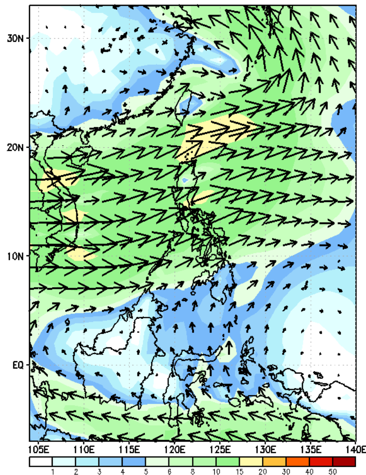
GEFS Week-1 850-hPa Wind Total Valid: 20230731 - 20230806
