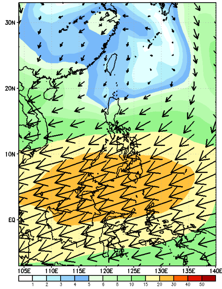
GEFS Week-1 200-hPa Wind Total Valid: 20230731 - 20230806
