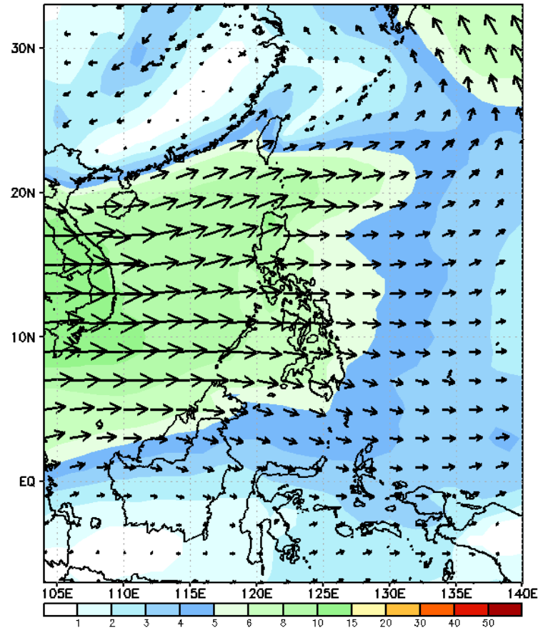
GEFS Week-2 700-hPa Wind Total Valid: 20230807 – 20230813
