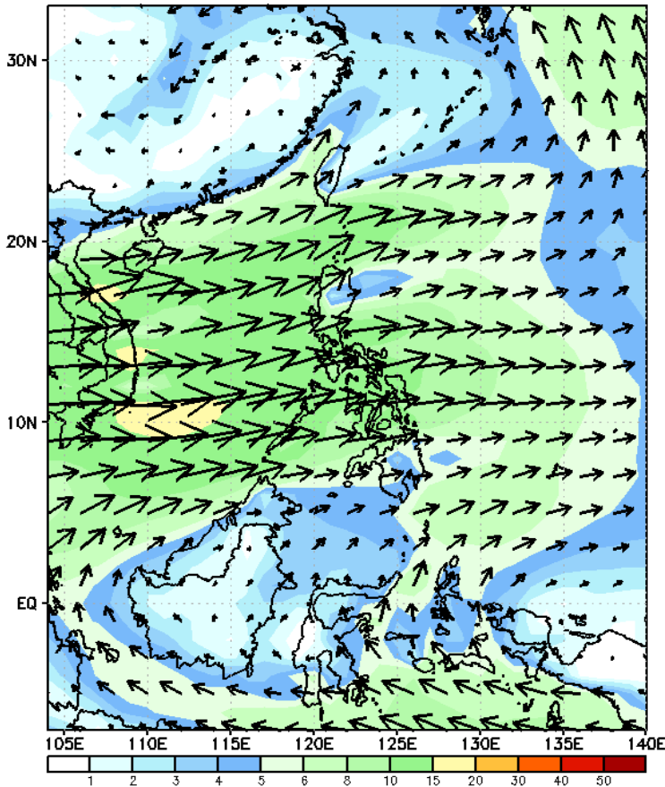
GEFS Week-2 850-hPa Wind Total Valid: 20230807 – 20230813
