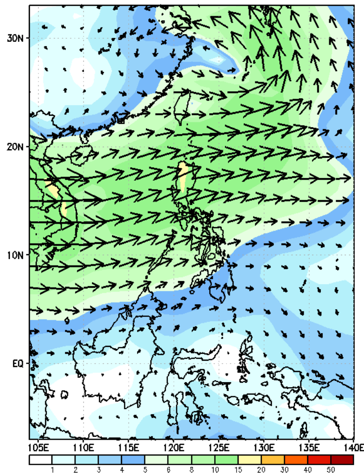
GEFS Week-1 700-hPa Wind Total Valid: 20230731 - 20230806
