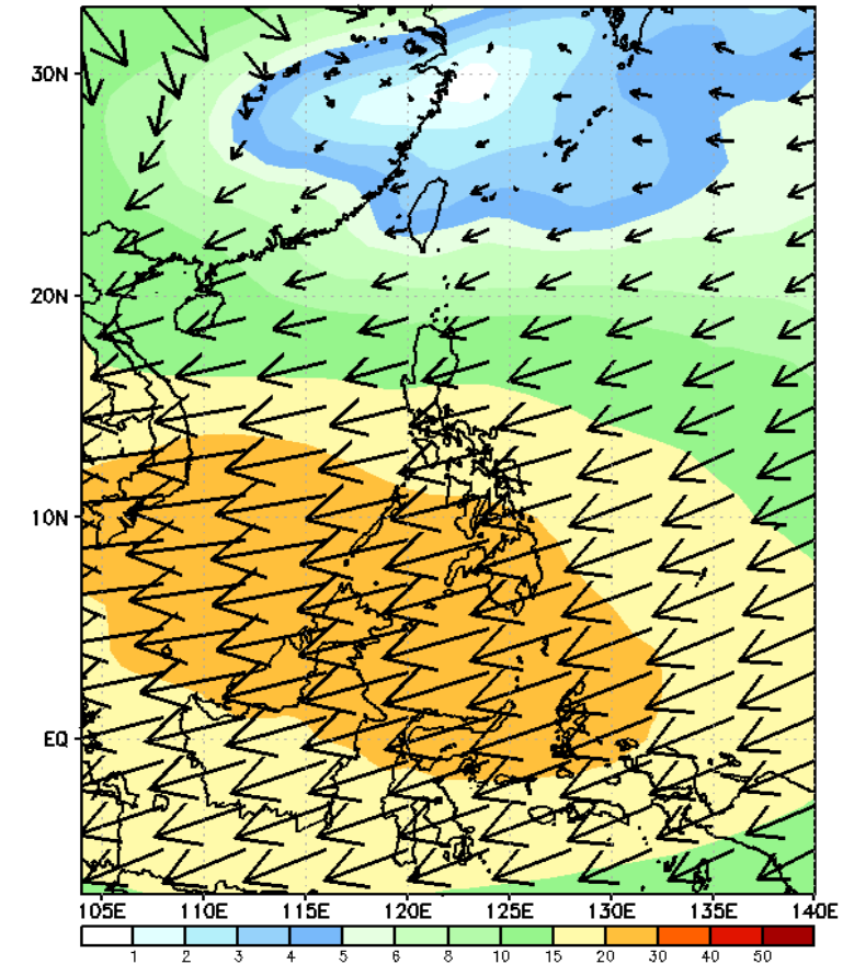
GEFS Week-2 200-hPa Wind Total Valid: 20230807 – 20230813
