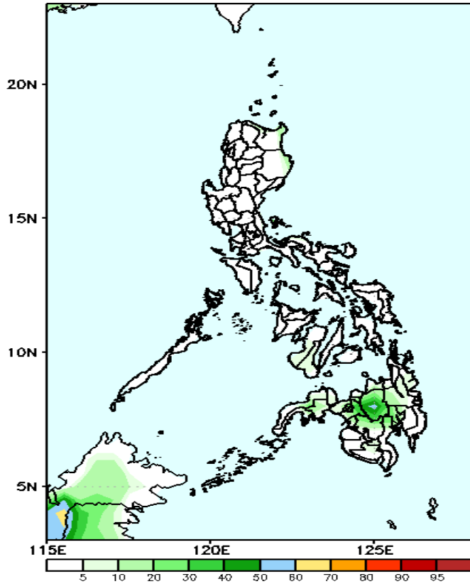
GEFS Week-1 Exceedance Prob. > 100mm Valid: 20231016 - 20231022
