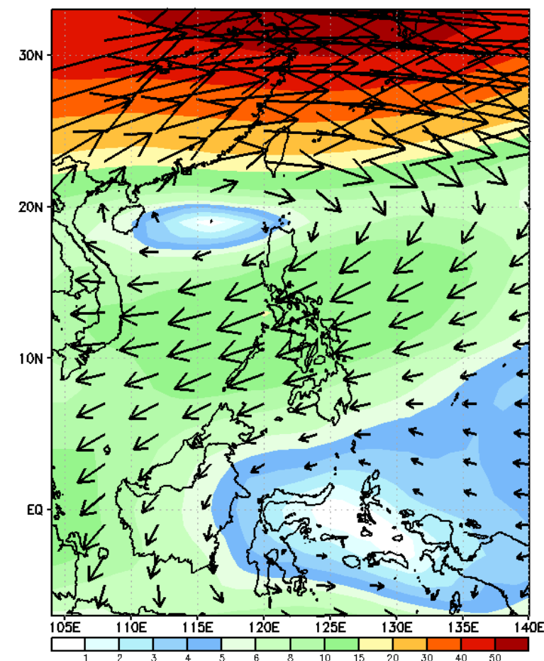
GEFS Week-1 200-hPa Wind Total Valid: 20231016 - 20231022
