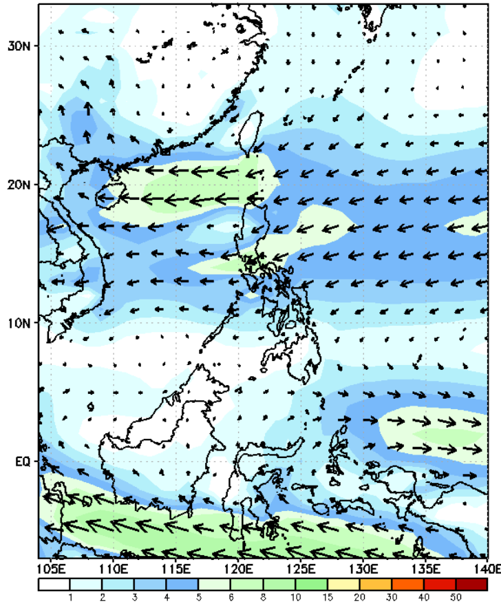
GEFS Week-2 850-hPa Wind Total Valid: 20231023 - 20231029
