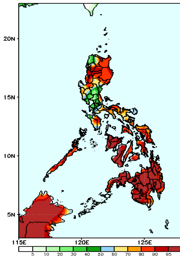
GEFS Week-1 Exceedance Prob. > 25mm Valid: 20231016 - 20231022
