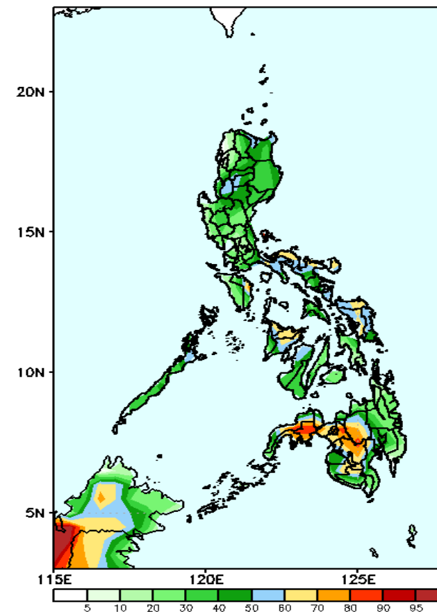
GEFS Week-2 Exceedance Prob. > 50mm Valid: 20231023 - 20231029
