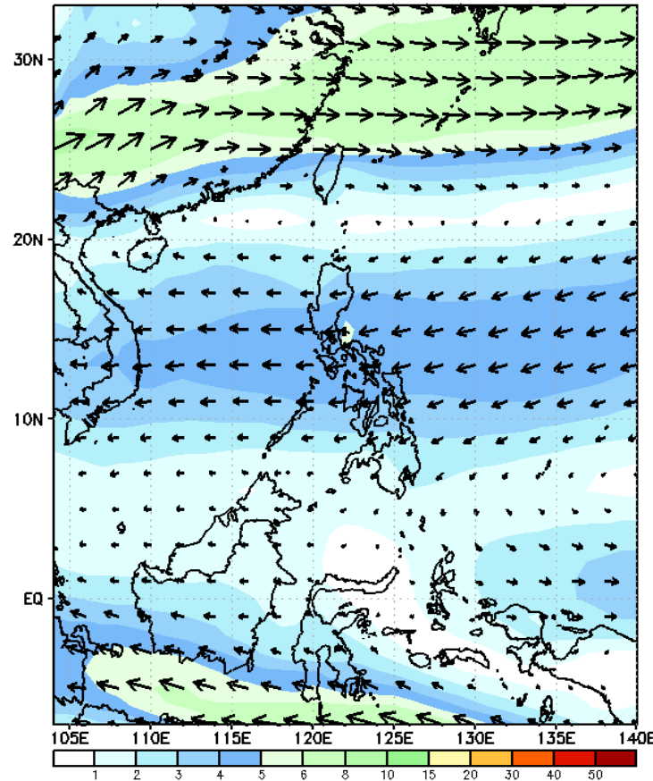
GEFS Week-2 700-hPa Wind Total Valid: 20231023 - 20231029
