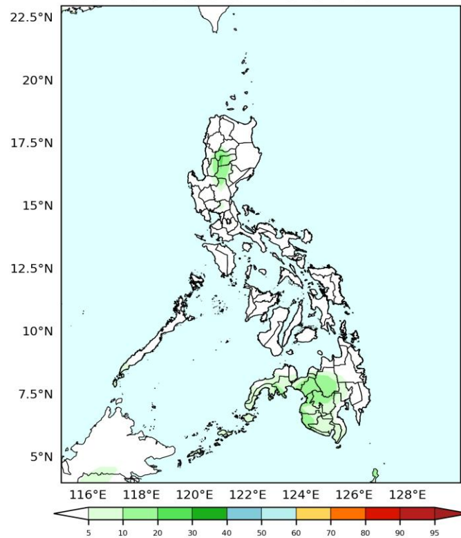
GEFS Week-2 Exceedance Prob. > 150mm
