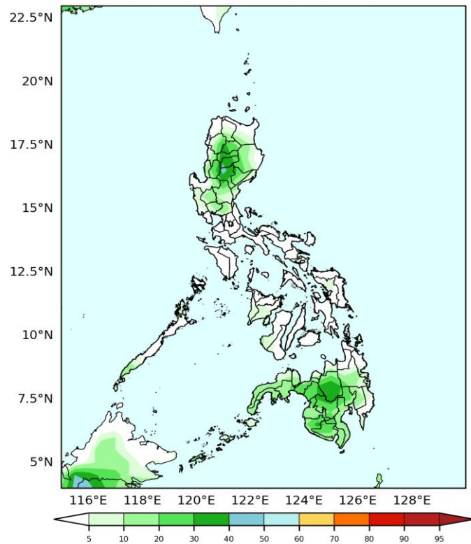
GEFS Week-2 Exceedance Prob. > 100mm
