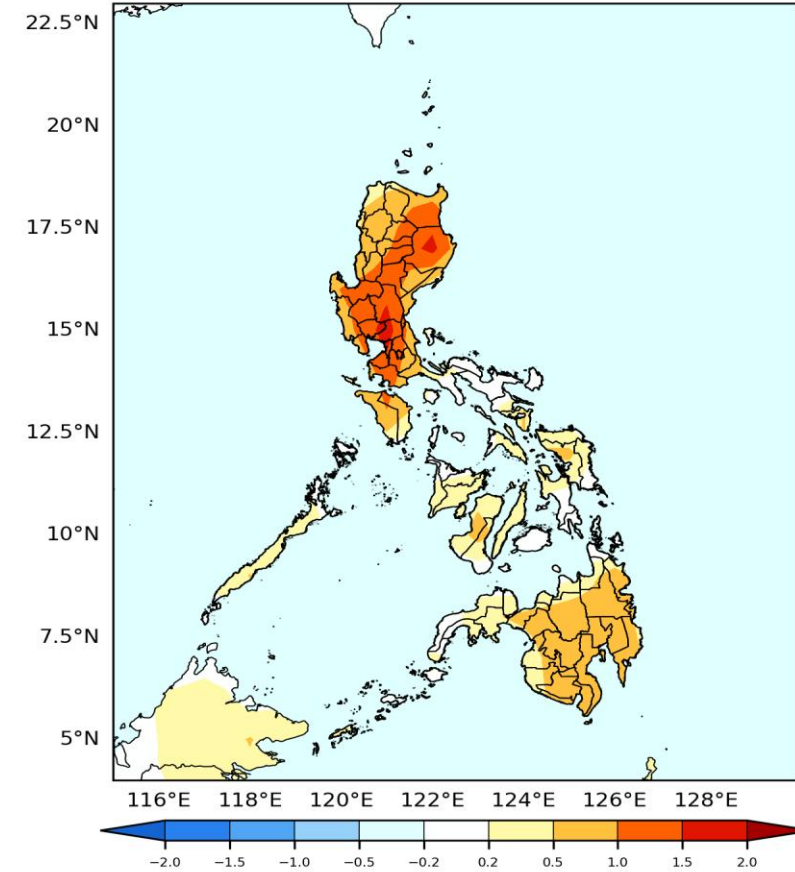
GEFS Week-2 T2m Anomaly
