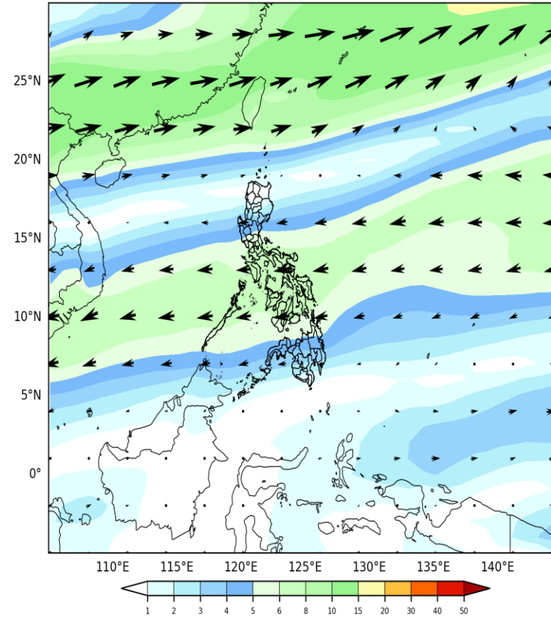
GEFS Week-1 700-hPa Wind Total
