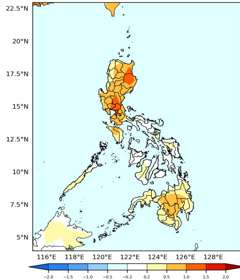
GEFS Week-2 T2m Anomaly Valid: 2026-05-07 to 2026-05-13
