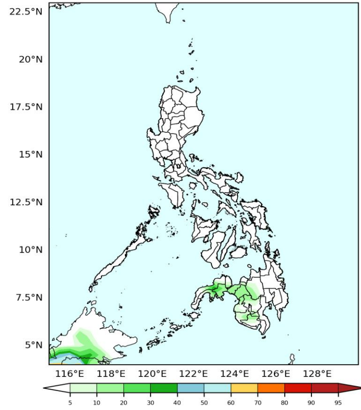
GEFS Week-1 Exceedance Prob. > 100mm
