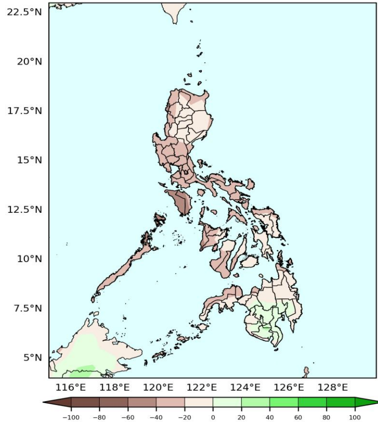
Precipitation Anomaly
