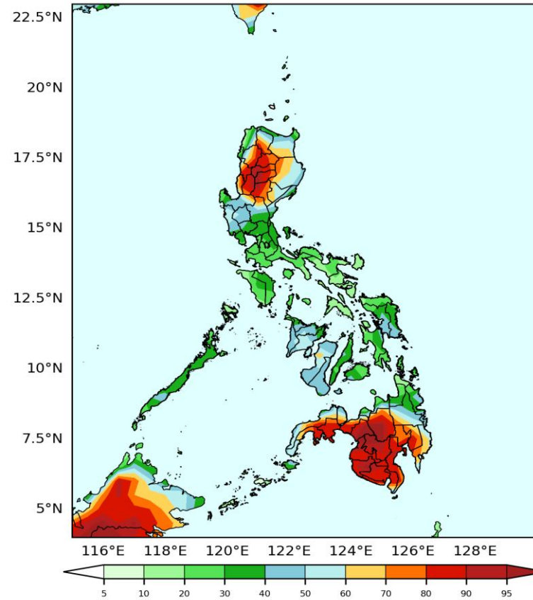
Probability to Exceed 25mm
