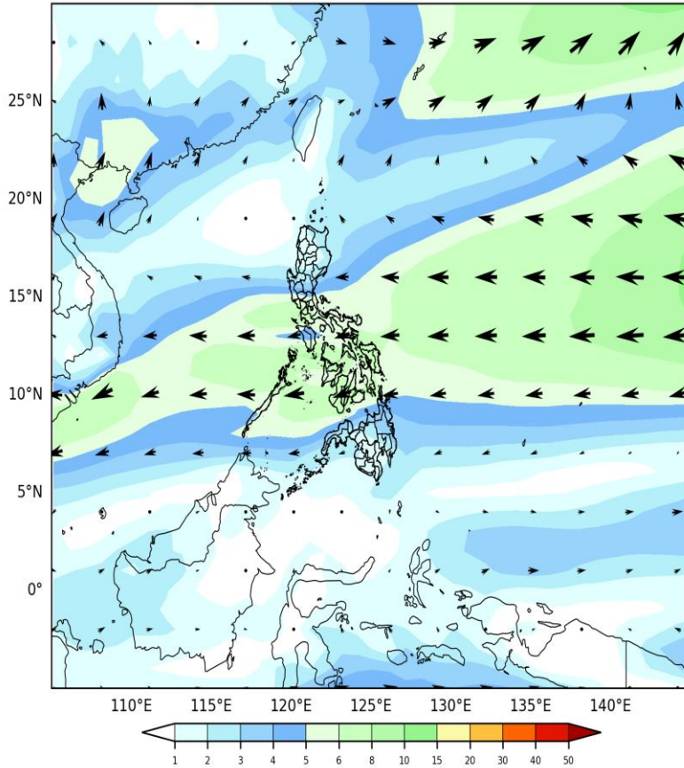
GEFS Week-1 850-hPa Wind Total
