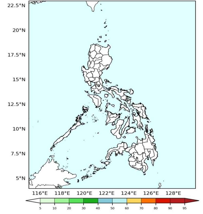
GEFS Week-2 Exceedance Prob. > 200mm Valid: 2026-05-07 to 2026-05-13
