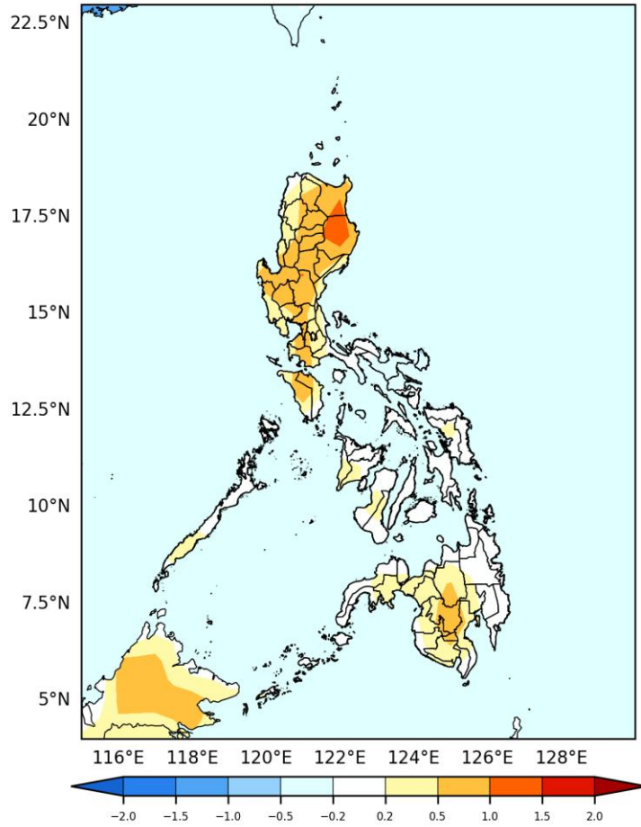
GEFS Week-1 T2m Anomaly Valid: 2026-04-30 to 2026-05-06
