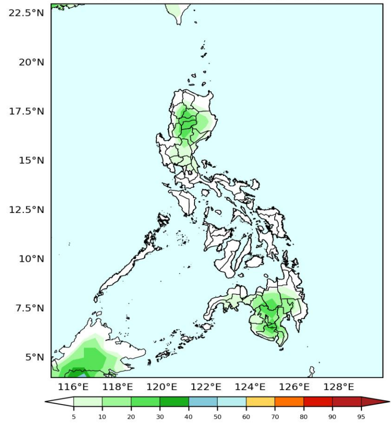
GEFS Week-2 Exceedance Prob. > 100mm Valid: 2026-05-07 to 2026-05-13
