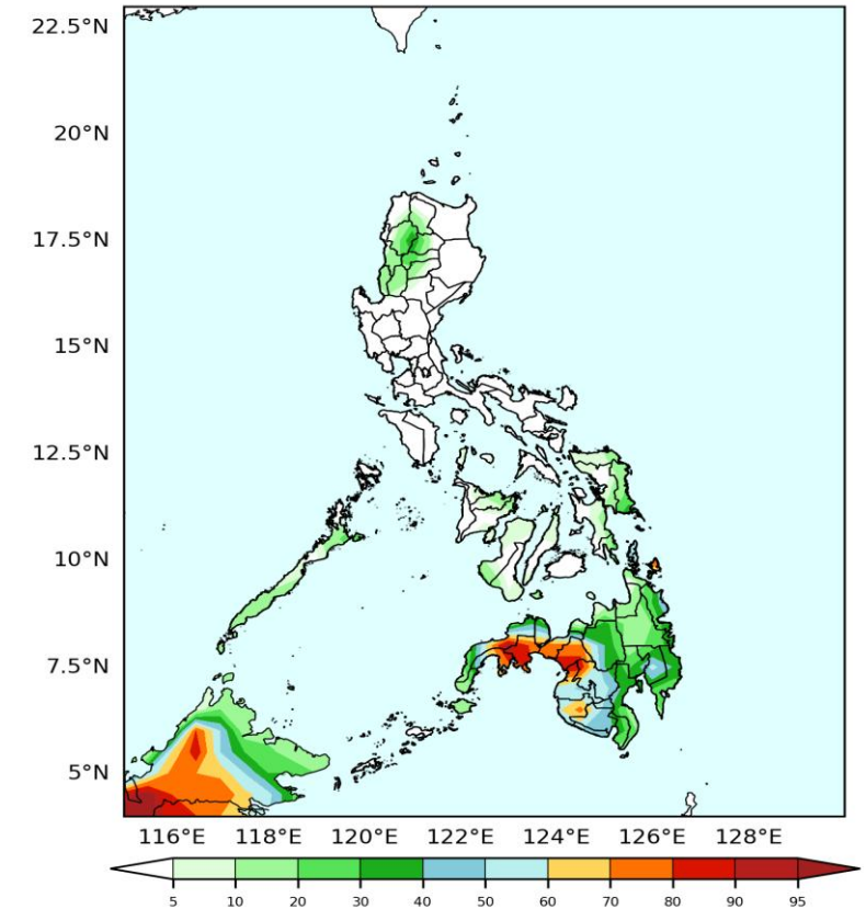
GEFS Week-1 Exceedance Prob. > 50mm
