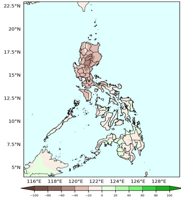
GEFS Week-1 Precip Anomaly
