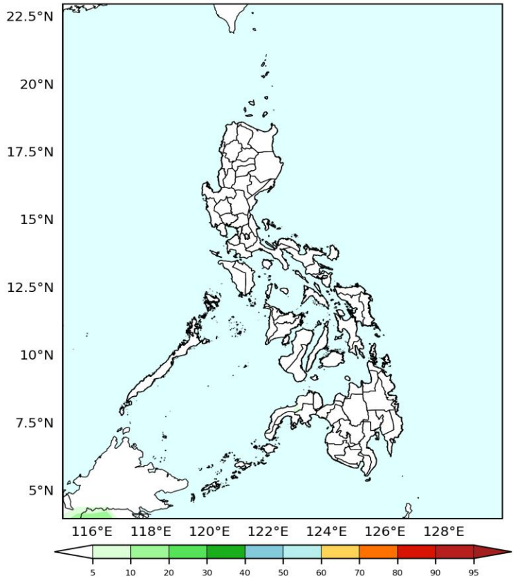
GEFS Week-1 Exceedance Prob. > 150mm
