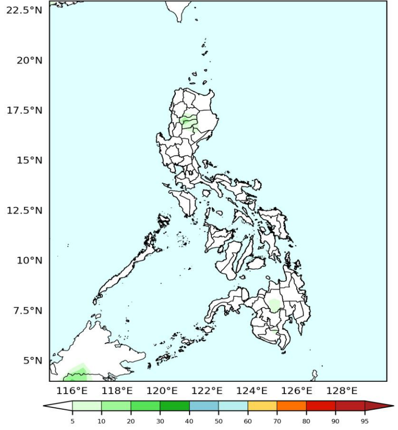
GEFS Week-2 Exceedance Prob. > 150mm Valid: 2026-05-07 to 2026-05-13
