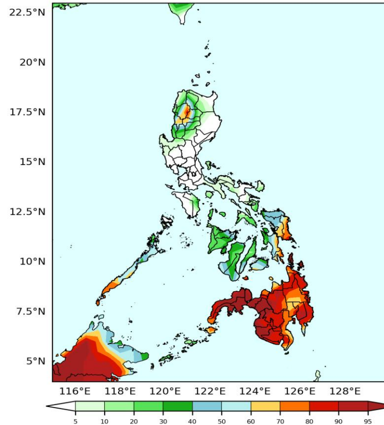
GEFS Week-1 Exceedance Prob. > 25mm
