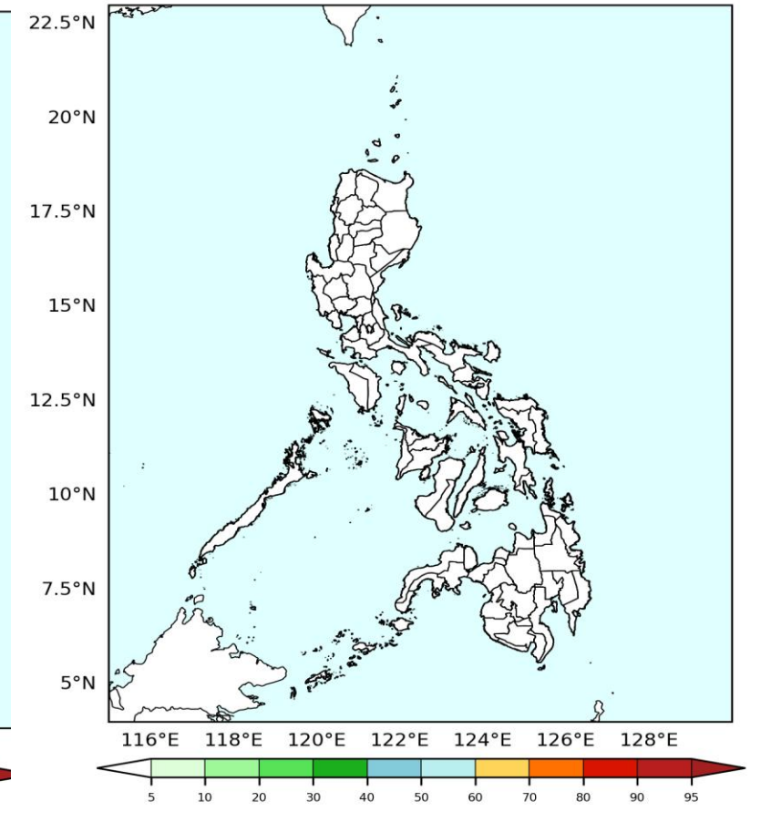
GEFS Week-2 Exceedance Prob. > 200mm Valid: 2026-04-23 to 2026-04-29
