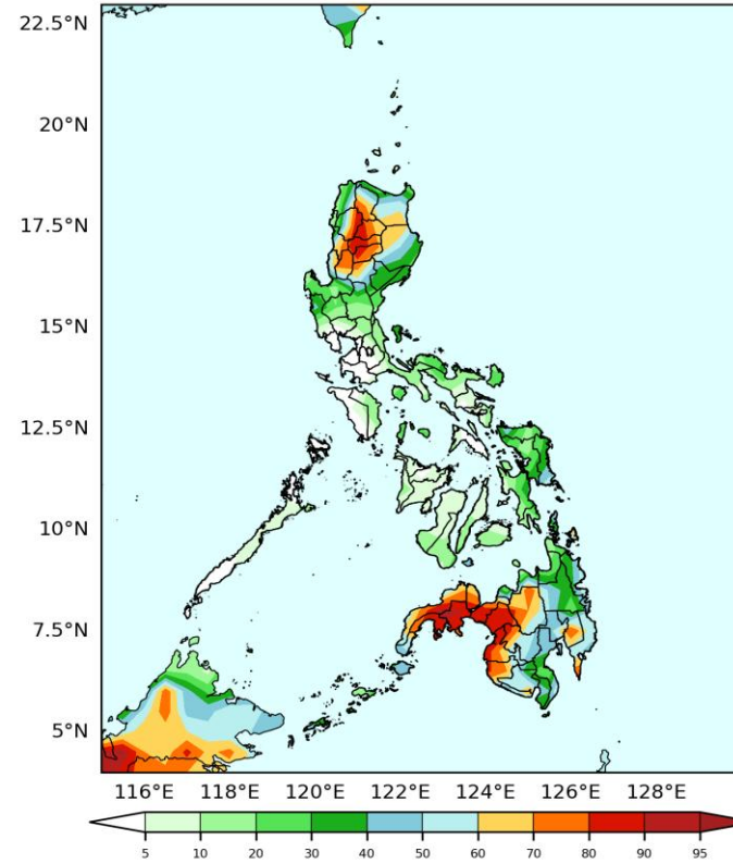
GEFS Week-2 Exceedance Prob. > 25mm
