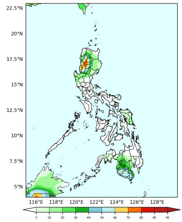
GEFS Week-1 Exceedance Prob. > 25mm Valid: 2026-04-16 to 2026-04-22
