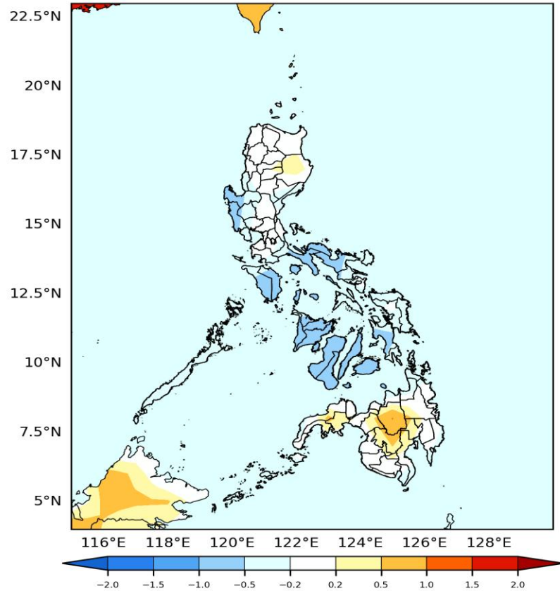
GEFS Week-1 T2m Anomaly
