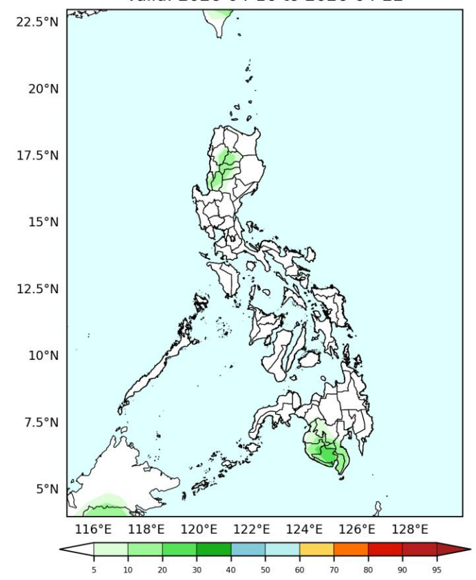
GEFS Week-1 Exceedance Prob. > 50mm Valid: 2026-04-16 to 2026-04-22
