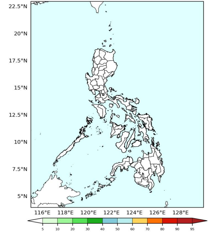
GEFS Week-1 Exceedance Prob. > 100mm Valid: 2026-04-16 to 2026-04-22
