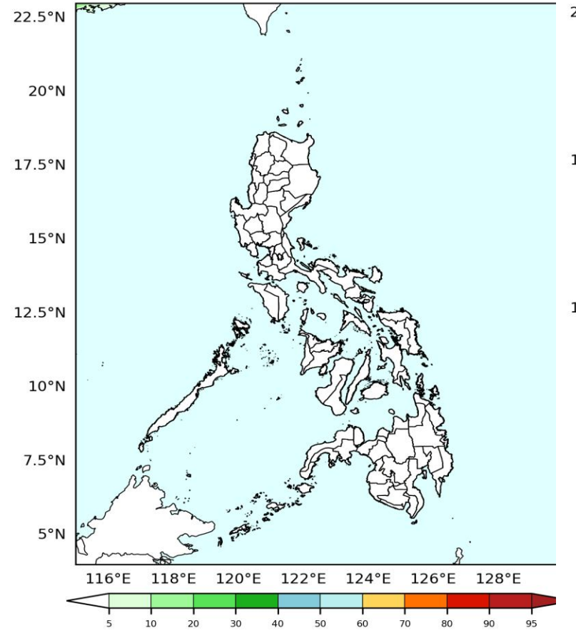
GEFS Week-2 Exceedance Prob. > 150mm Valid: 2026-04-23 to 2026-04-29
