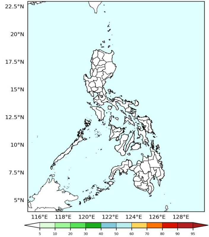
GEFS Week-1 Exceedance Prob. > 200mm Valid: 2026-04-16 to 2026-04-22
