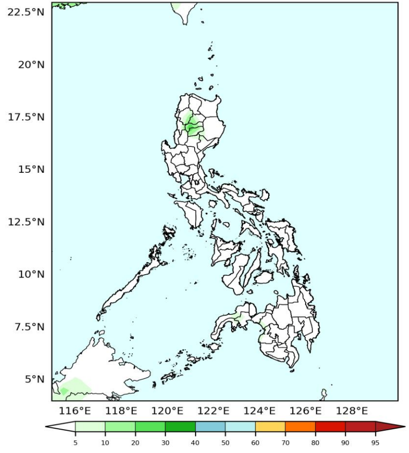
GEFS Week-2 Exceedance Prob. > 100mm Valid: 2026-04-23 to 2026-04-29
