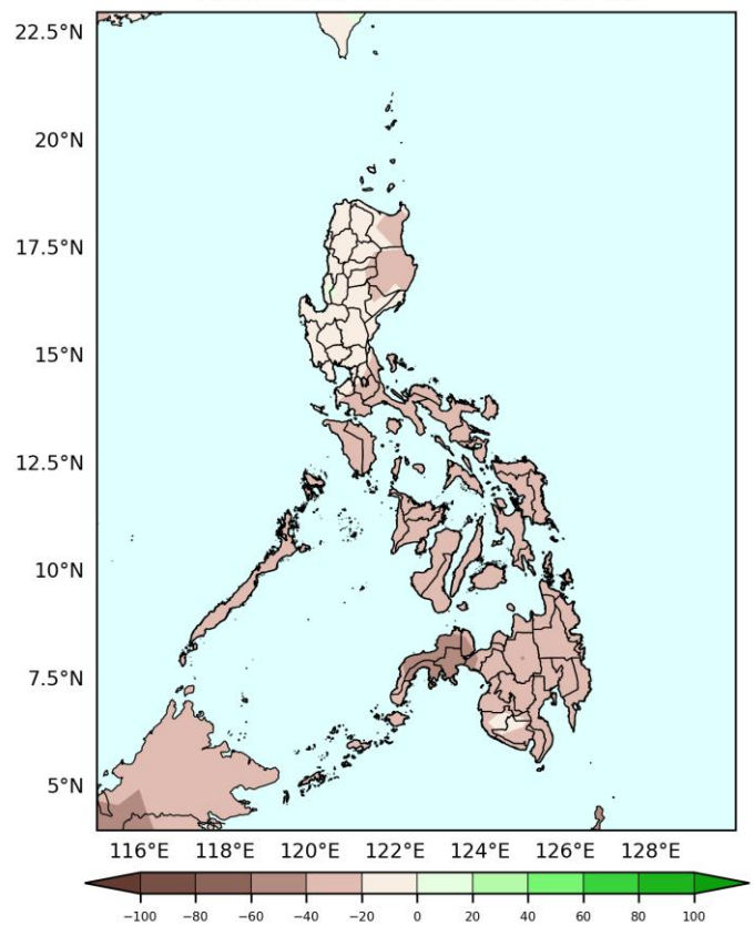
GEFS Week-1 Precip Anomaly Valid: 2026-04-16 to 2026-04-22
