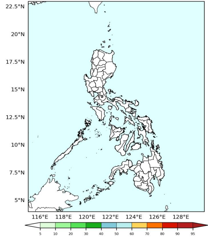
GEFS Week-1 Exceedance Prob. > 150mm Valid: 2026-04-16 to 2026-04-22
