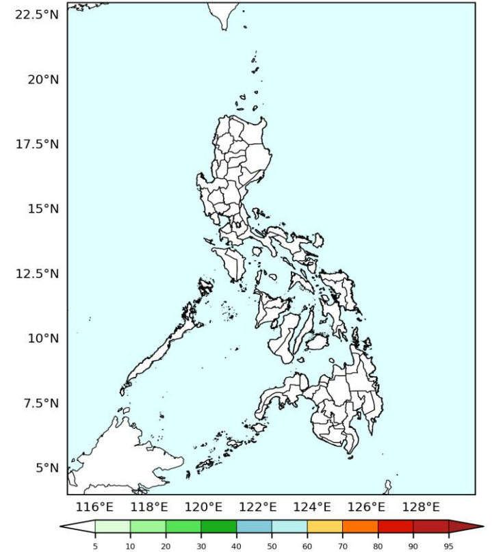
GEFS Week-1 Exceedance Prob. > 200mm Valid: 2026-03-30 to 2026-04-05
