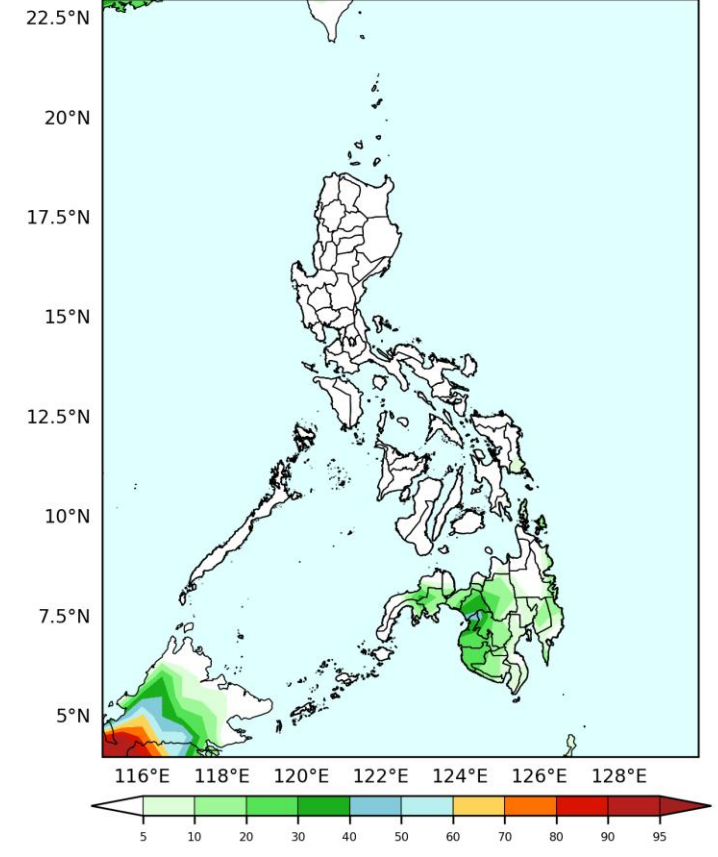
GEFS Week-1 Exceedance Prob. > 50mm Valid: 2026-03-30 to 2026-04-05
