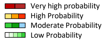
GEFS Week-1 Exceedance Prob. > 50mm Valid: 2026-03-30 to 2026-04-05
