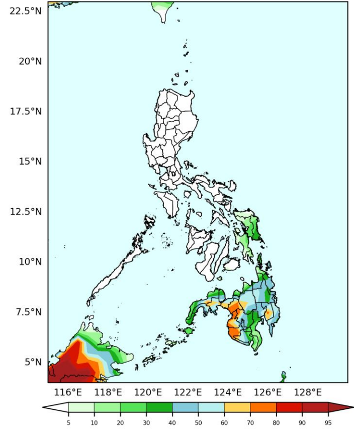
GEFS Week-1 Exceedance Prob. > 25mm Valid: 2026-03-30 to 2026-04-05
