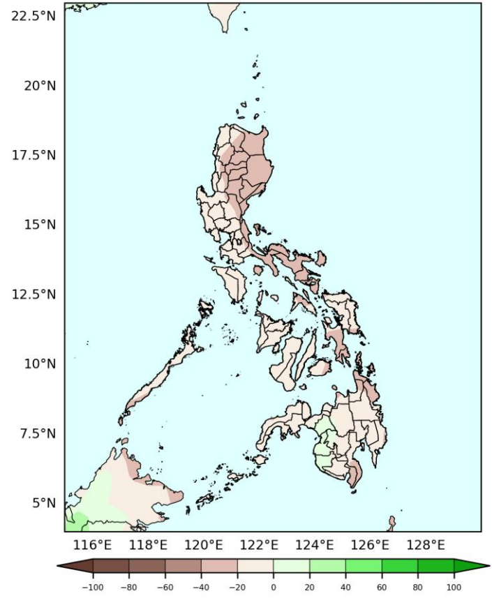
GEFS Week-1 Precip Anomaly Valid: 2026-03-30 to 2026-04-05
