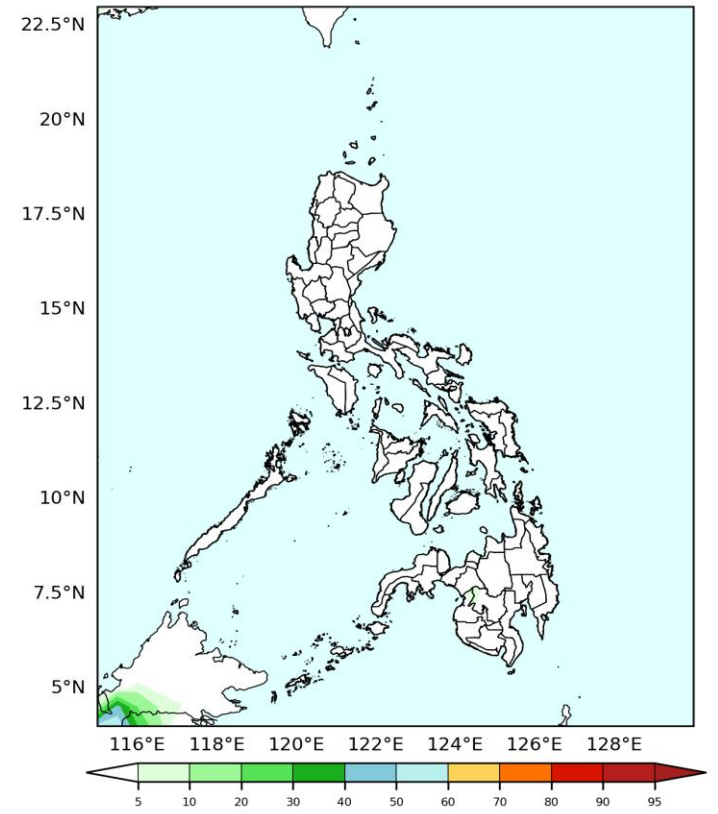
GEFS Week-1 Exceedance Prob. > 100mm Valid: 2026-03-30 to 2026-04-05
