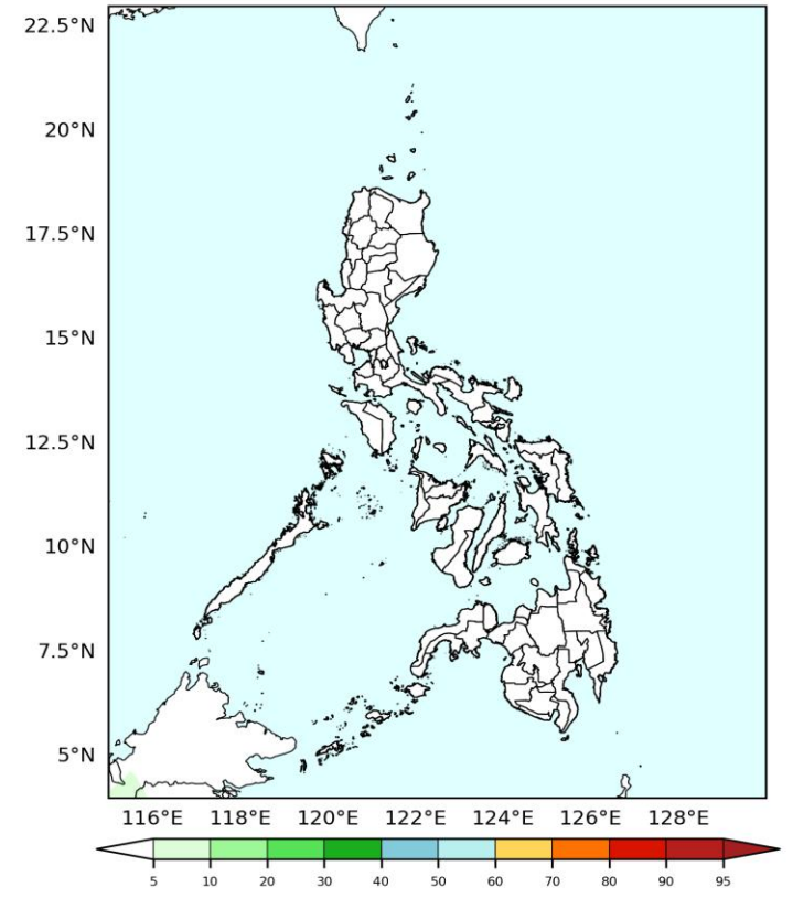
GEFS Week-1 Exceedance Prob. > 150mm Valid: 2026-03-30 to 2026-04-05
