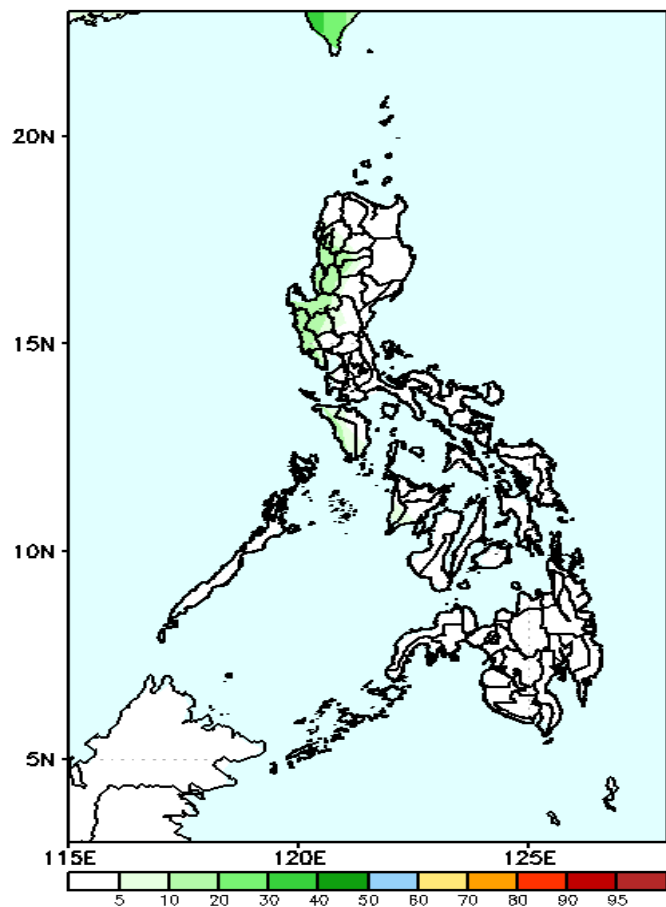
GEFS Week-2 Exceedance Prob. > 200mm Valid: 20210805 – 20210811
