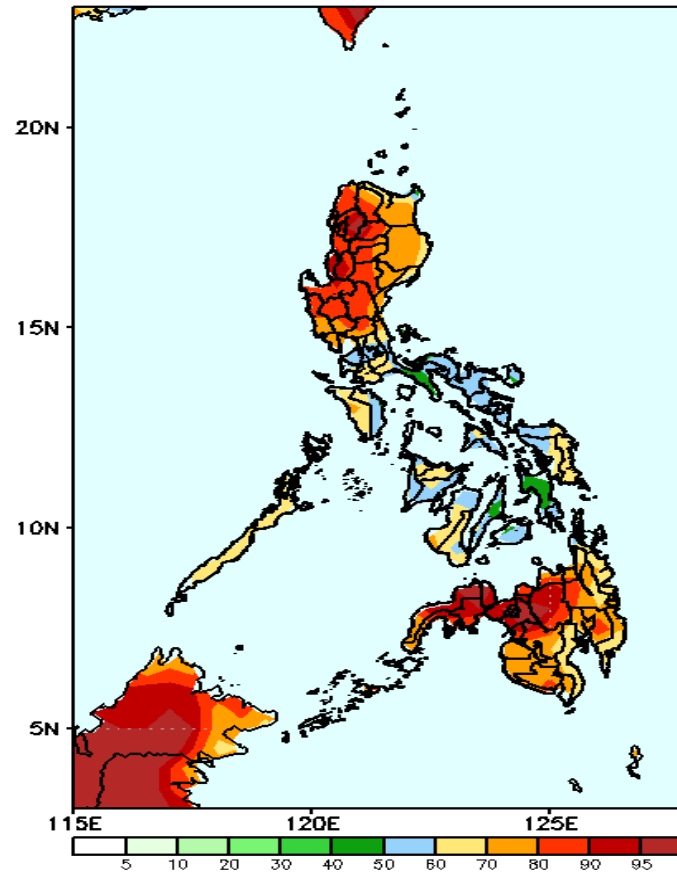
GEFS Week-2 Exceedance Prob. > 25m Valid: 20210805 - 20210811
