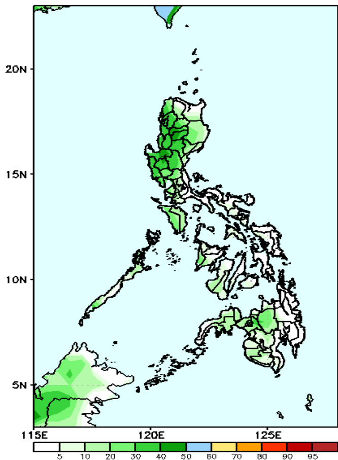
GEFS Week-2 Exceedance Prob. > 100mm Valid: 20210805 – 20210811
