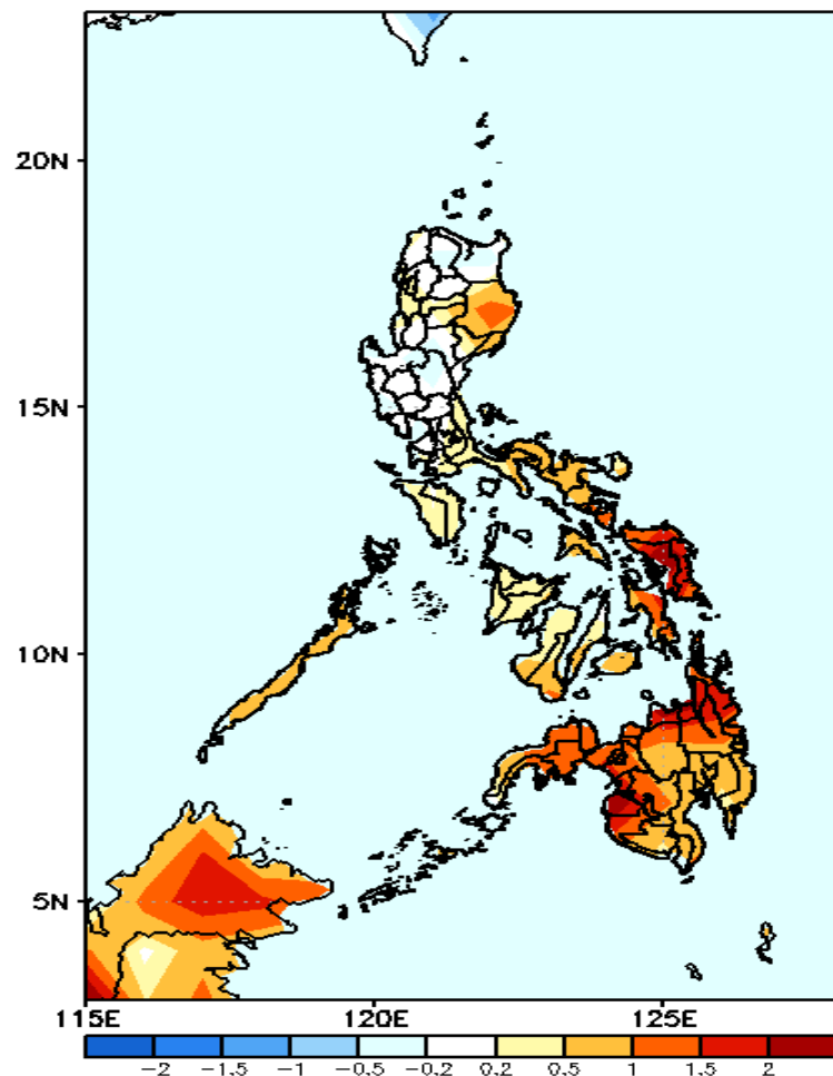
GEFS Week-1 T2m Anomaly Valid: 20210729 - 20210804
