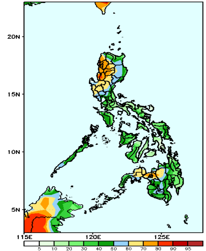
GEFS Week-2 Exceedance Prob. > 50mm Valid: 20210805 - 20210811
