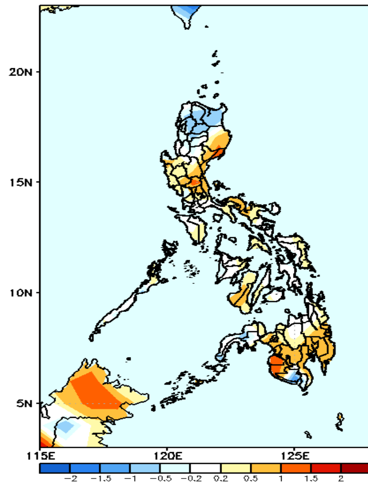
GEFS Week-2 T2m Anomaly Valid: 20210805 - 20210811
