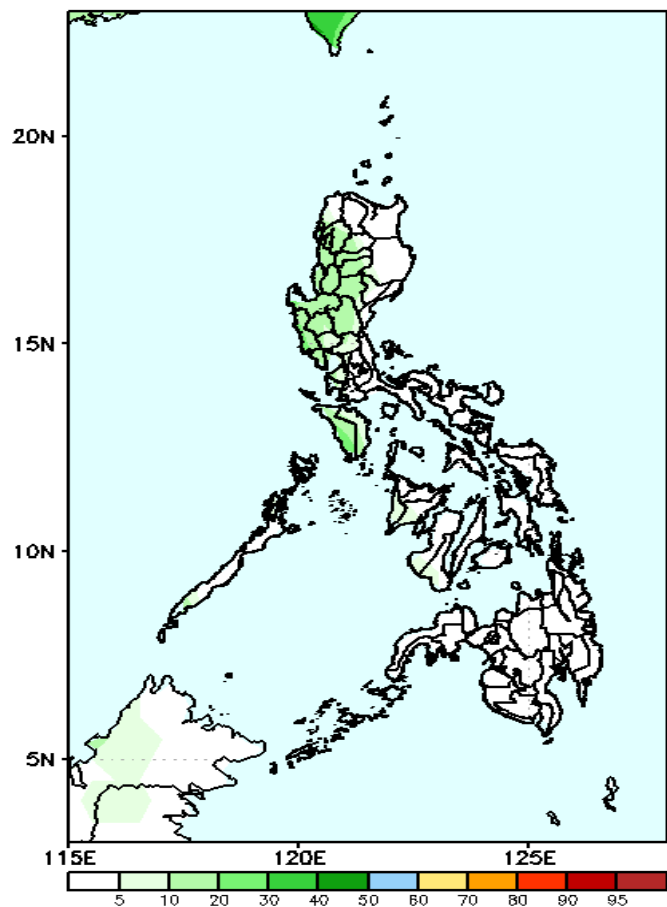
GEFS Week-2 Exceedance Prob. > 150mm Valid: 20210805 – 20210811
