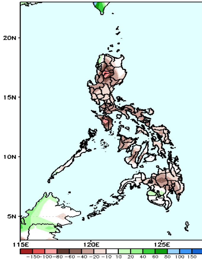
GEFS Week-2 Precip Anomaly Valid: 20210805 - 20210811
