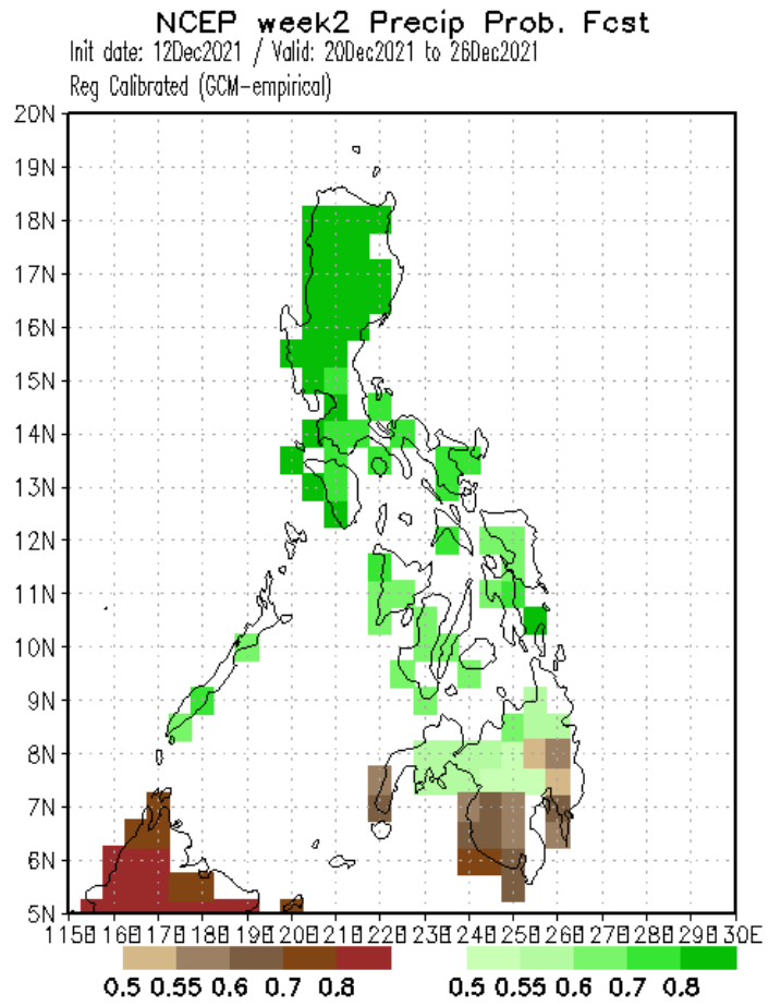
Probability of receiving above normal rainfall in most parts of the country except in southern Mindanao where below normal is more likely.
